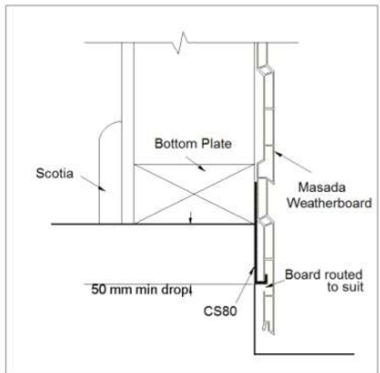
Fig 2 Half Drop Starting
