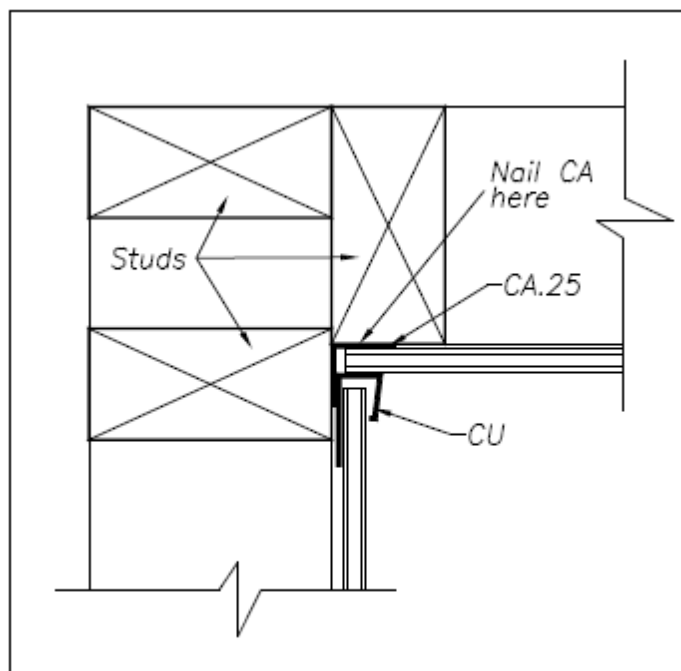
Fig 3b Alternative Internal Corner
