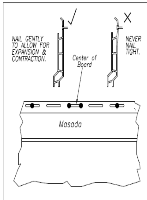
Fig 15 Fixing Details
