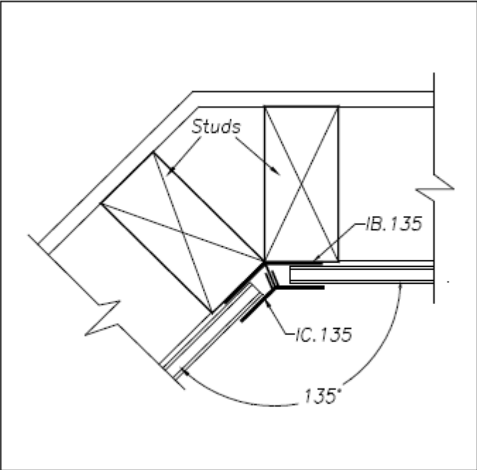
Fig 5 135° Internal Corner
