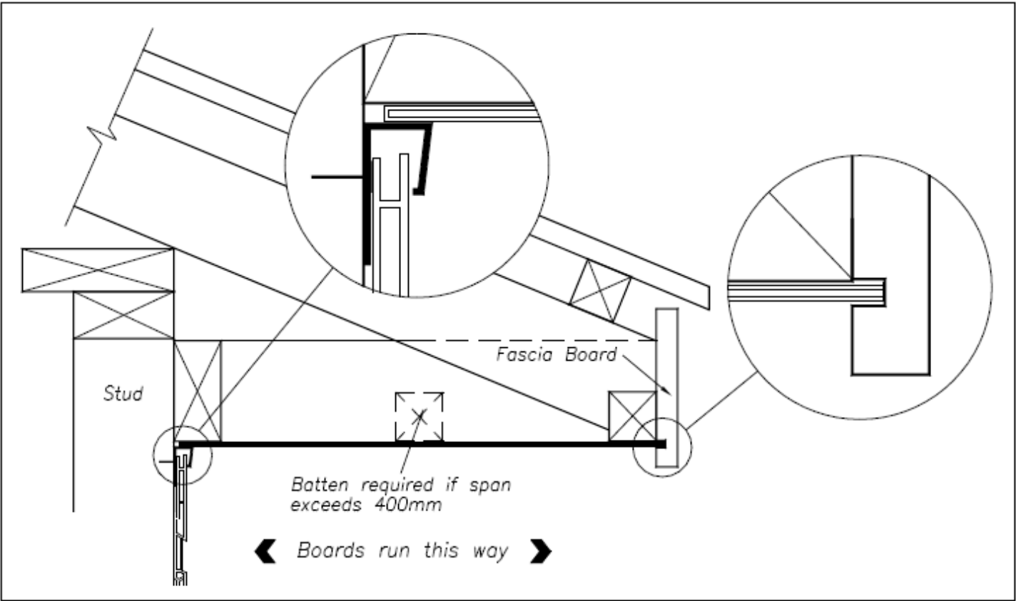
Fig 21 Soffit Detail
