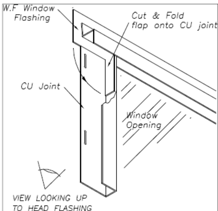
Fig 12 Head Flashing
