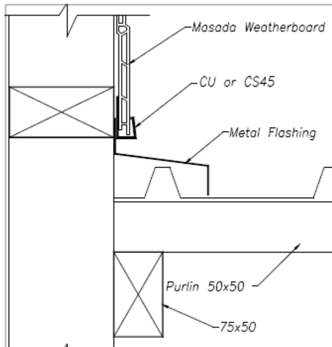
Fig 18 Roof Flashing
