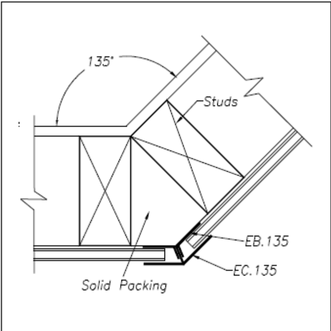
Fig 6 135° External Corner
