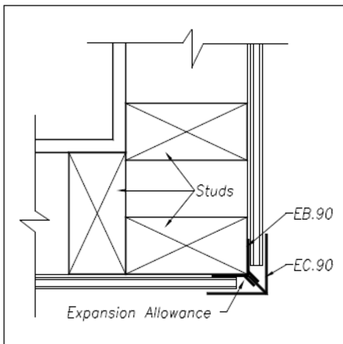
Fig 4 90° External Corner
