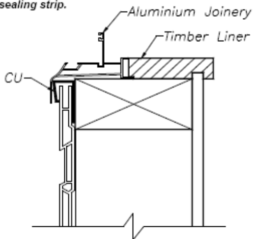
Fig 7 Sill
